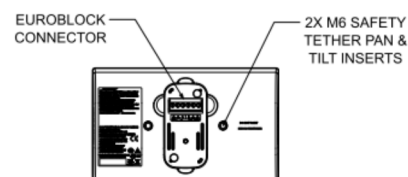
Rear View BRACKET ONLY
