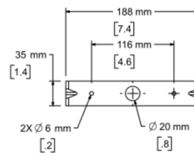
Rear View BRACKET ONLY
