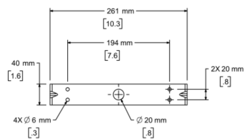
Rear View BRACKET ONLY
