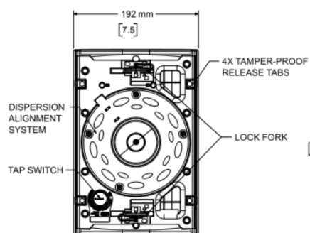
Front View GRILLE REMOVED FOR CLARITY
